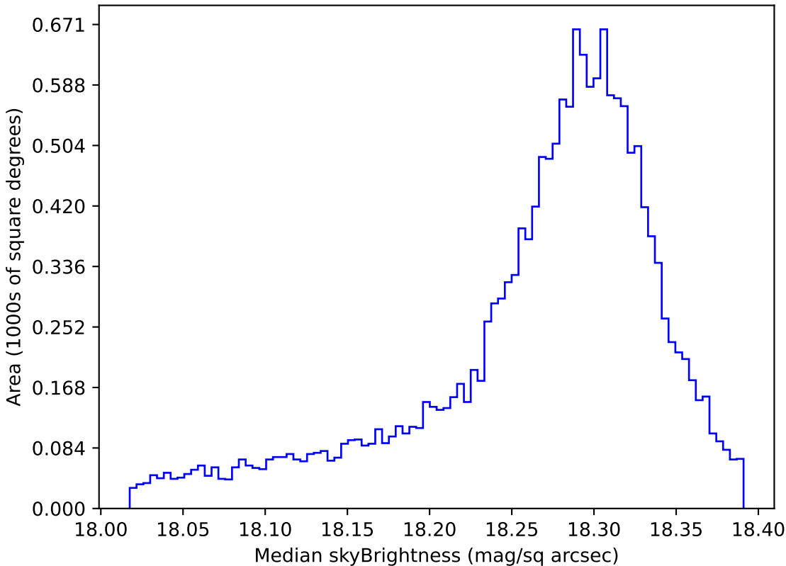
too_elab_r8_d2_gz_v3.4_10yrs WFD y band: Median skyBrightness
