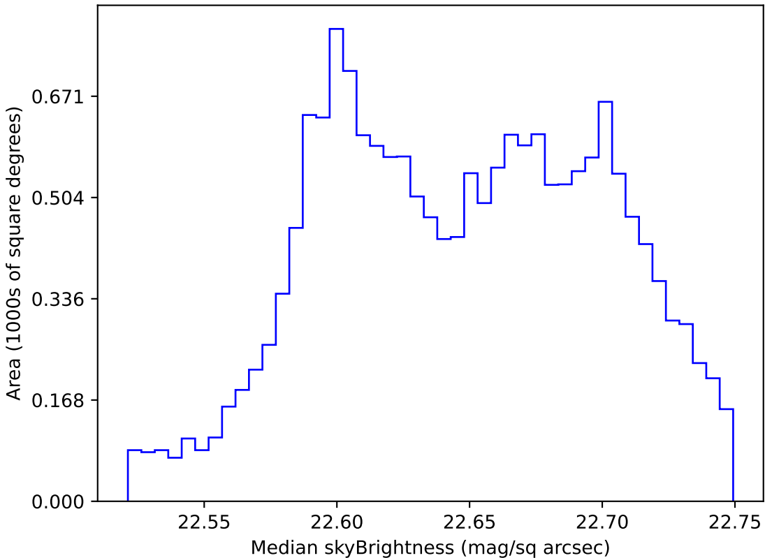
too_elab_r8_d2_gz_v3.4_10yrs WFD u band: Median skyBrightness
