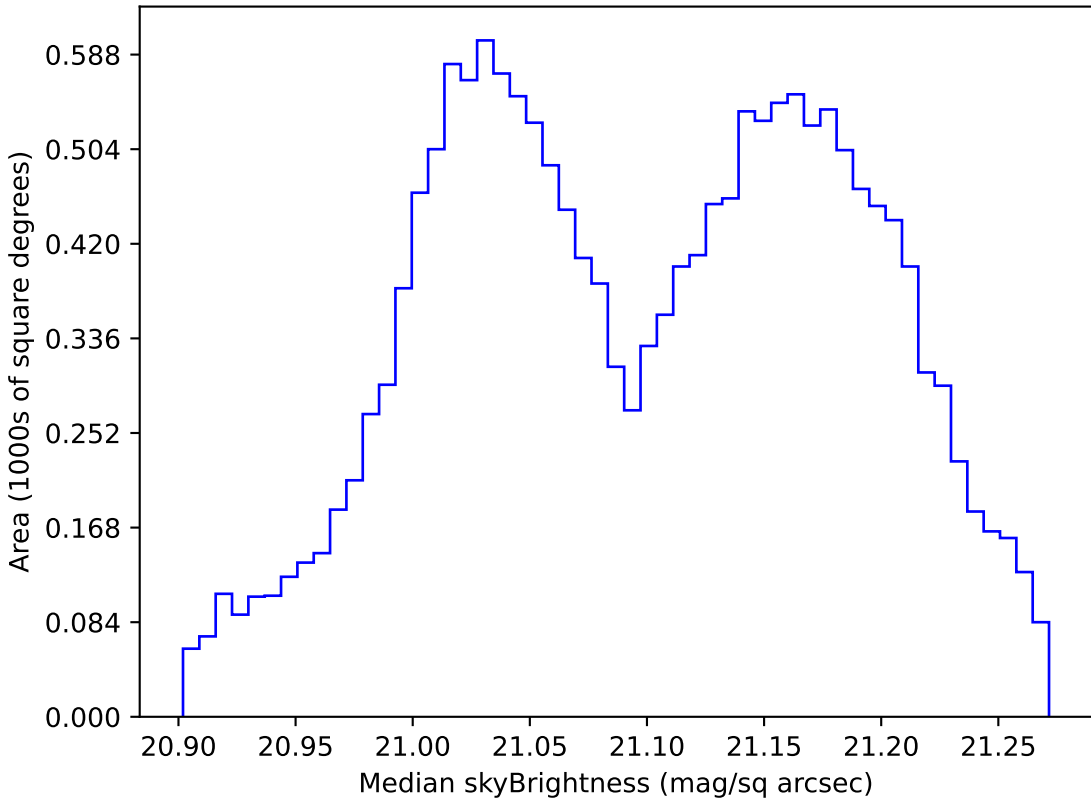
too_elab_r8_d2_gz_v3.4_10yrs WFD r band: Median skyBrightness
