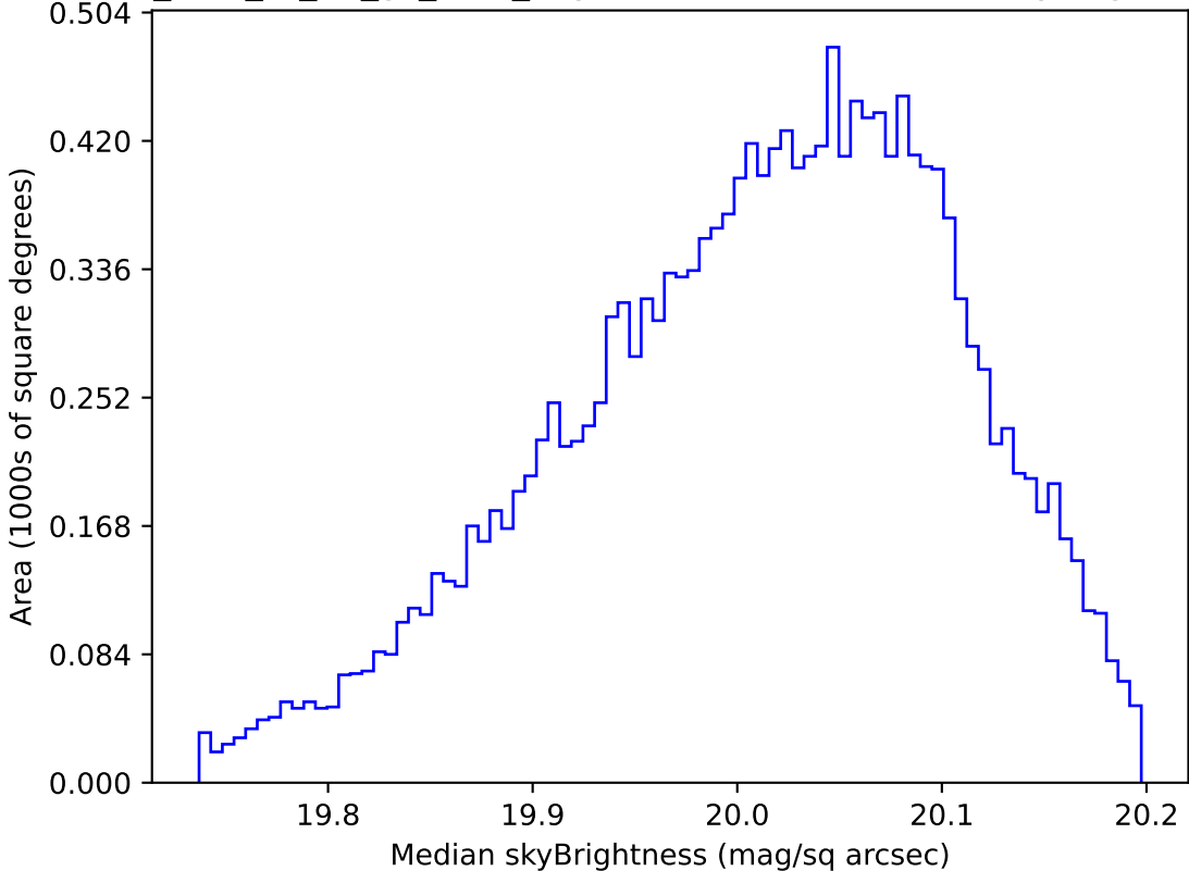
too_elab_r8_d2_gz_v3.4_10yrs WFD i band: Median skyBrightness
