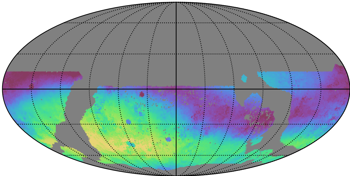
too_elab_r8_d2_gz_v3.4_10yrs WFD g band: Median skyBrightness
