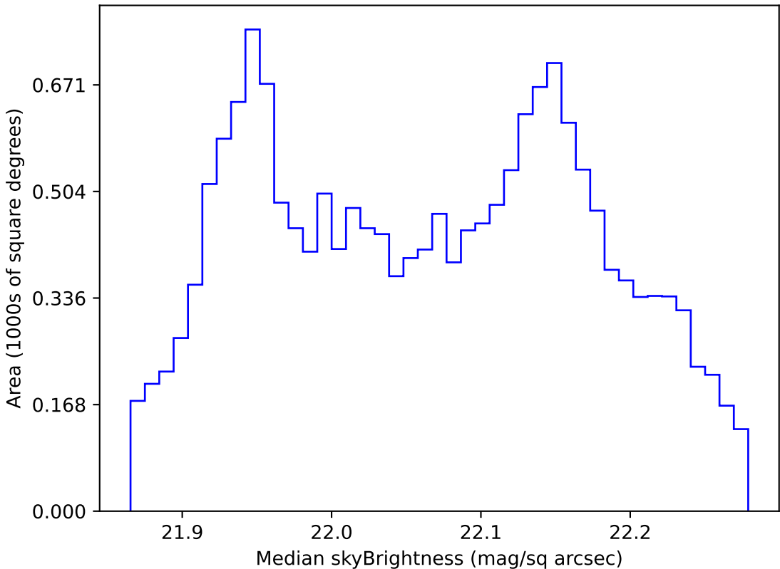
too_elab_r8_d2_gz_v3.4_10yrs WFD g band: Median skyBrightness
