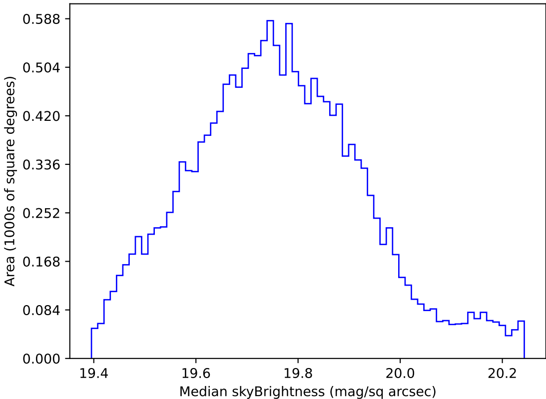
too_elab_r8_d2_gz_v3.4_10yrs WFD all bands: Median skyBrightness
