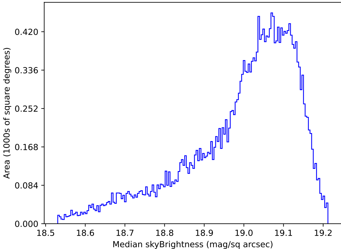
too_elab_r8_d2_gz_v3.4_10yrs All sky z band: Median skyBrightness
