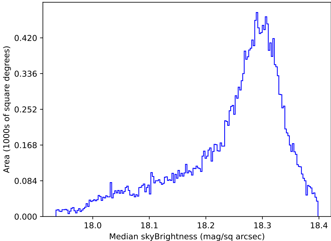
too_elab_r8_d2_gz_v3.4_10yrs All sky y band: Median skyBrightness
