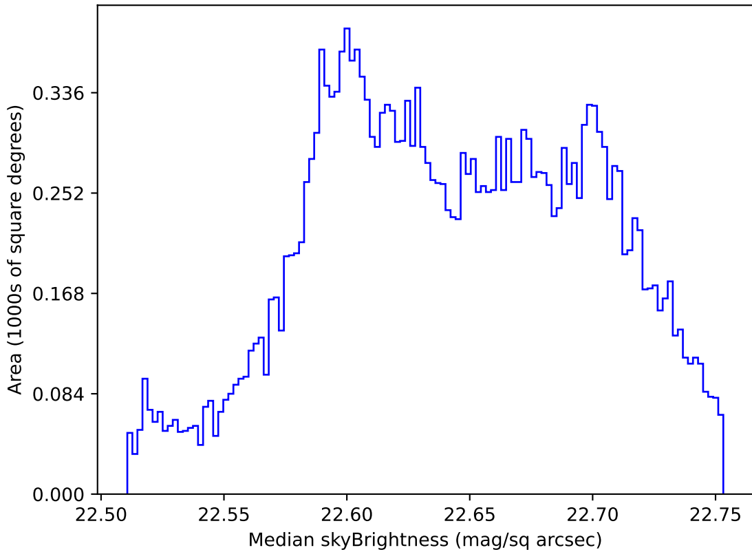
too_elab_r8_d2_gz_v3.4_10yrs All sky u band: Median skyBrightness
