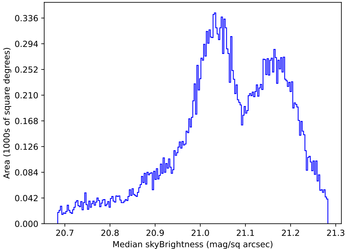
too_elab_r8_d2_gz_v3.4_10yrs All sky r band: Median skyBrightness
