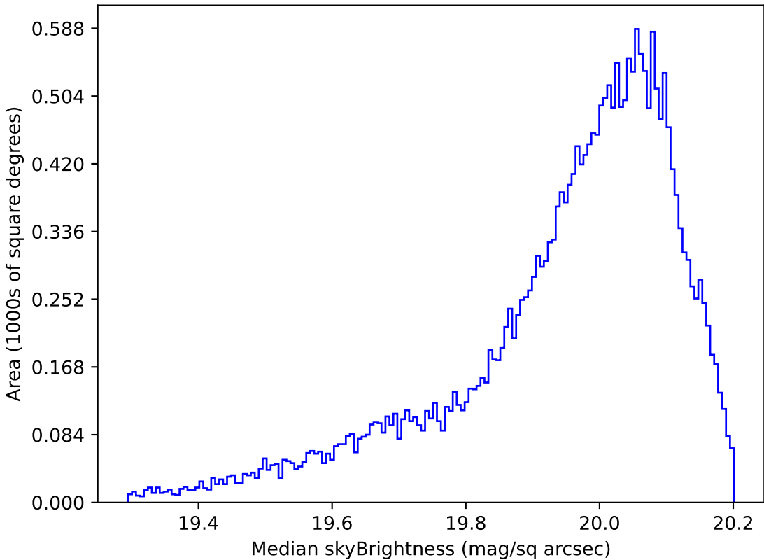
too_elab_r8_d2_gz_v3.4_10yrs All sky i band: Median skyBrightness
