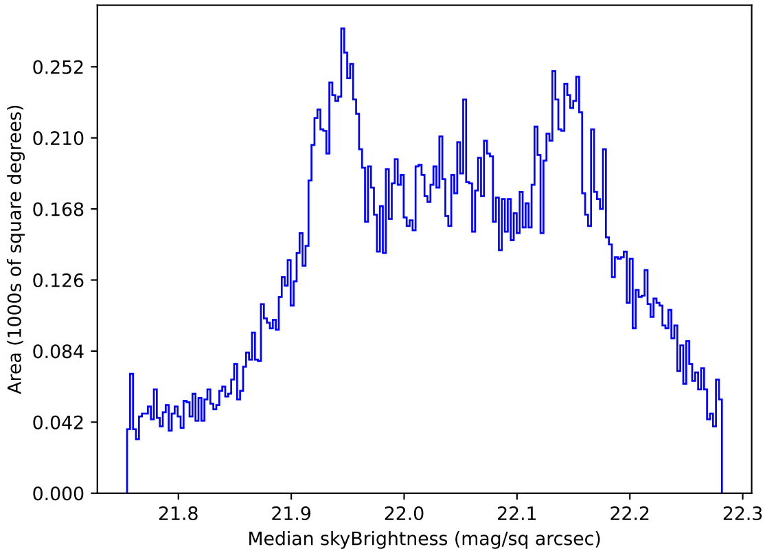
too_elab_r8_d2_gz_v3.4_10yrs All sky g band: Median skyBrightness
