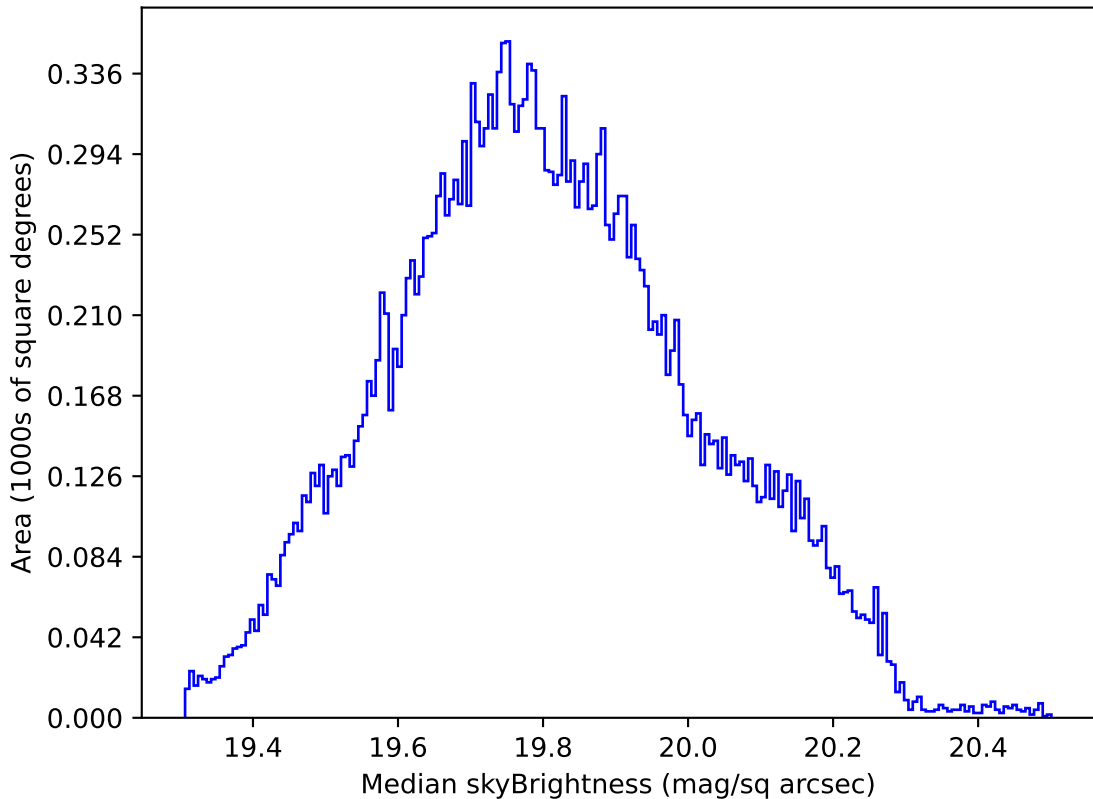
too_elab_r8_d2_gz_v3.4_10yrs All sky all bands: Median skyBrightness
