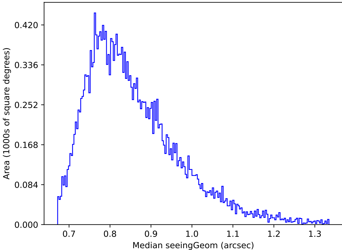
too_elab_r8_d2_gz_v3.4_10yrs Yr 1 z band: Median seeingGeom
