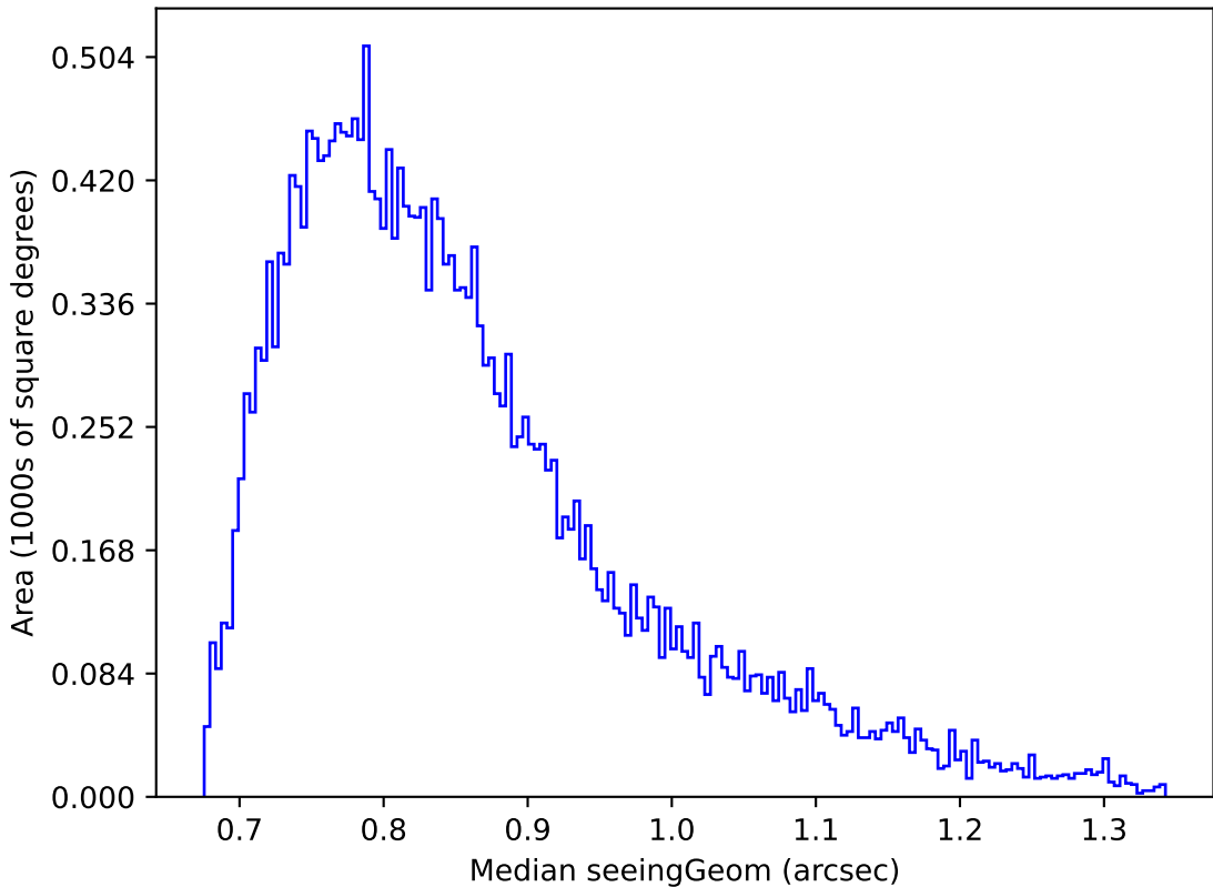
too_elab_r8_d2_gz_v3.4_10yrs Yr 1 r band: Median seeingGeom
