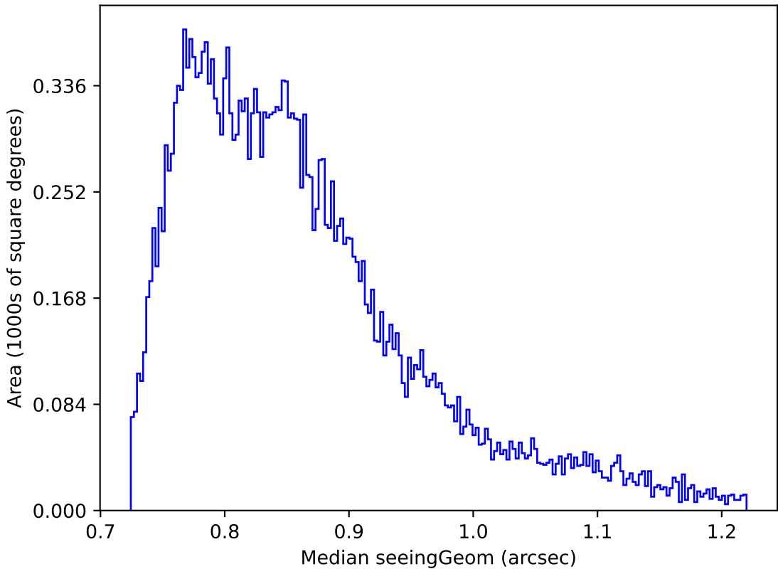
too_elab_r8_d2_gz_v3.4_10yrs Yr 1 all bands: Median seeingGeom
