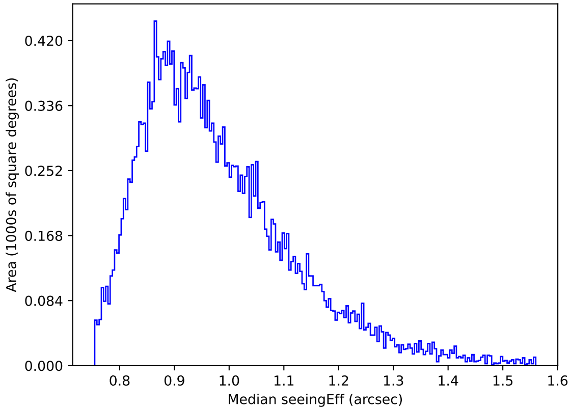
too_elab_r8_d2_gz_v3.4_10yrs Yr 1 z band: Median seeingEff
