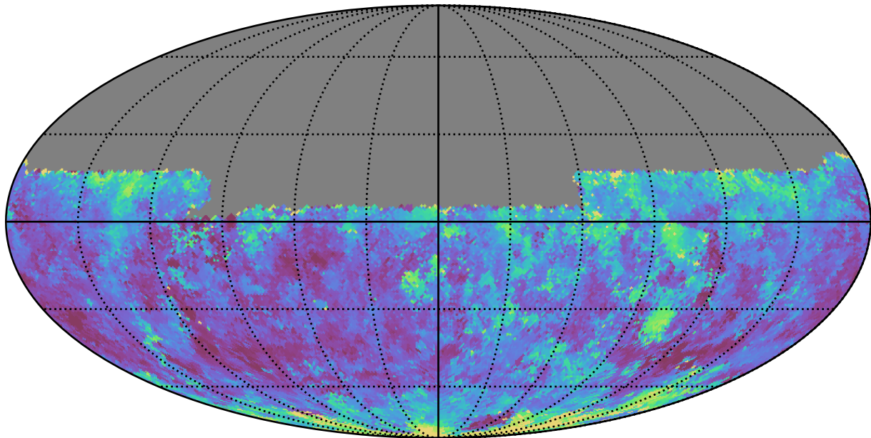
too_elab_r8_d2_gz_v3.4_10yrs Yr 1 y band: Median seeingEff
