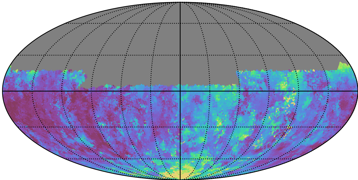
too_elab_r8_d2_gz_v3.4_10yrs Yr 1 u band: Median seeingEff
