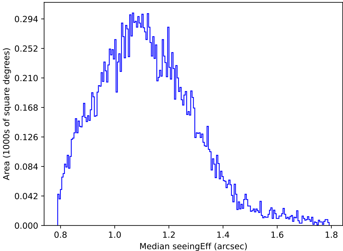
too_elab_r8_d2_gz_v3.4_10yrs Yr 1 u band: Median seeingEff
