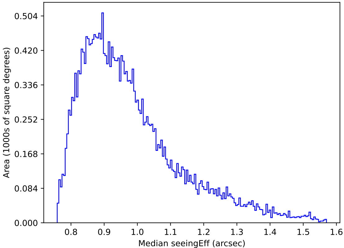
too_elab_r8_d2_gz_v3.4_10yrs Yr 1 r band: Median seeingEff
