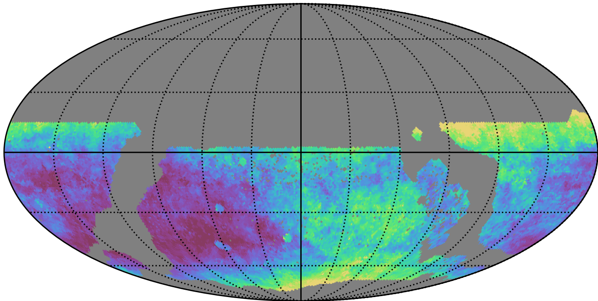
too_elab_r8_d2_gz_v3.4_10yrs WFD z band: Median seeingEff
