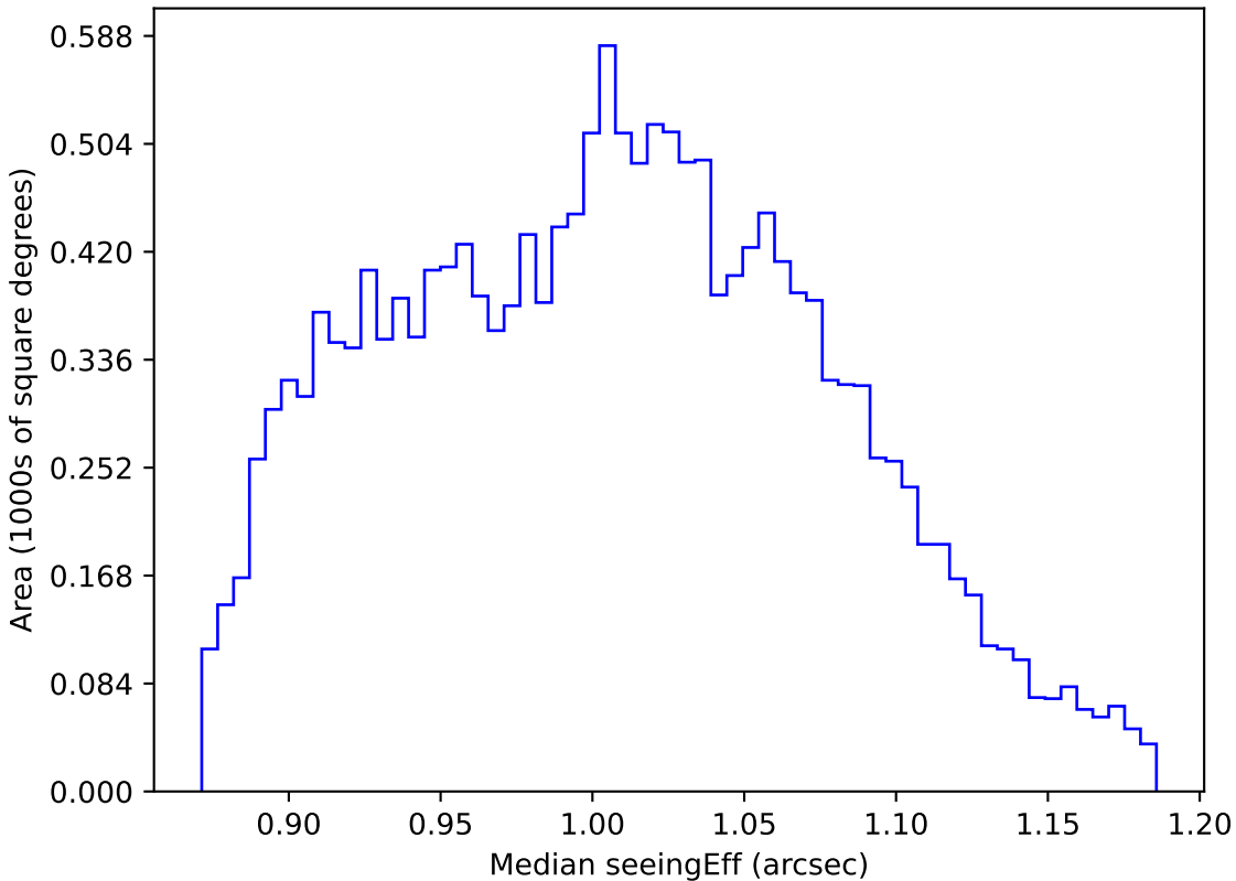
too_elab_r8_d2_gz_v3.4_10yrs WFD z band: Median seeingEff
