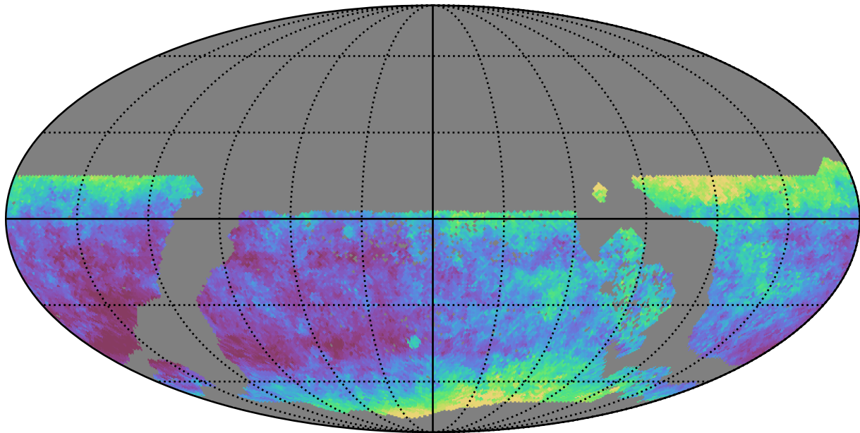
too_elab_r8_d2_gz_v3.4_10yrs WFD y band: Median seeingEff
