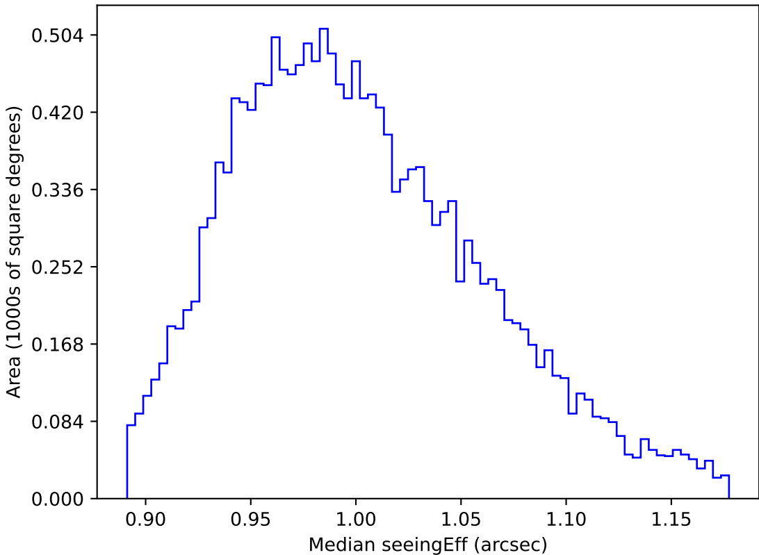
too_elab_r8_d2_gz_v3.4_10yrs WFD y band: Median seeingEff
