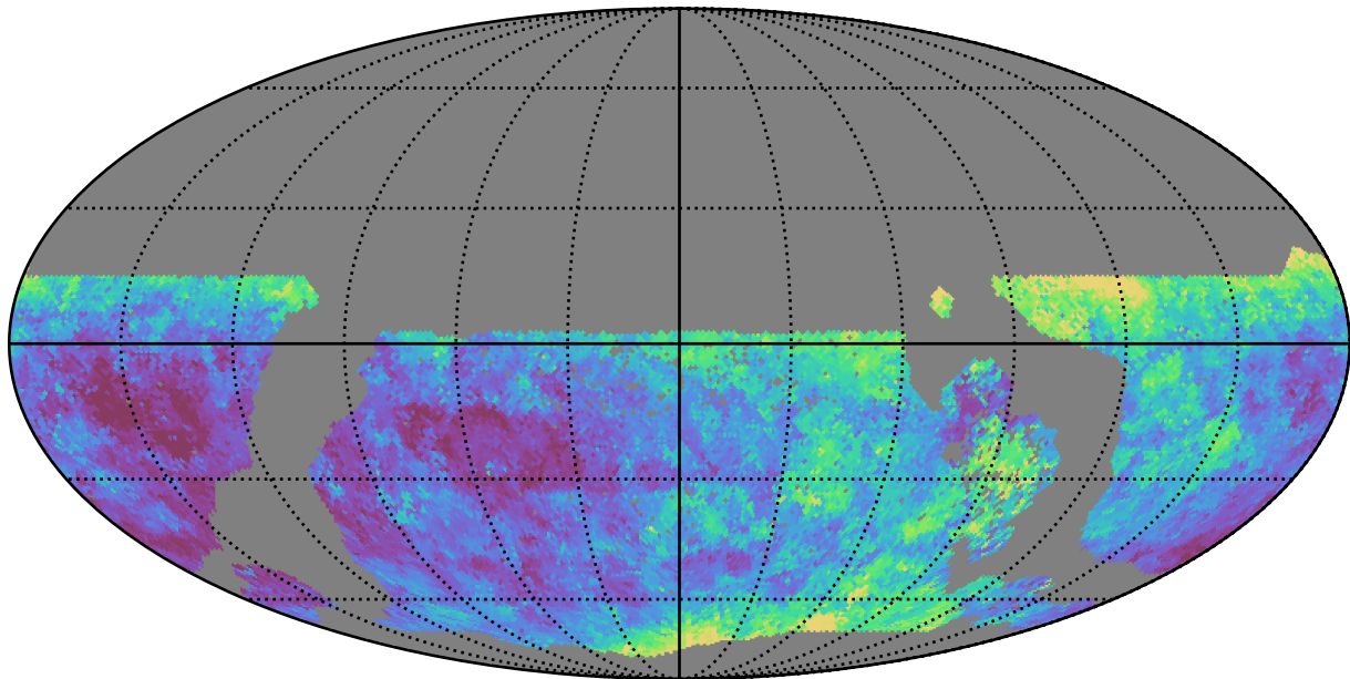
too_elab_r8_d2_gz_v3.4_10yrs WFD u band: Median seeingEff
