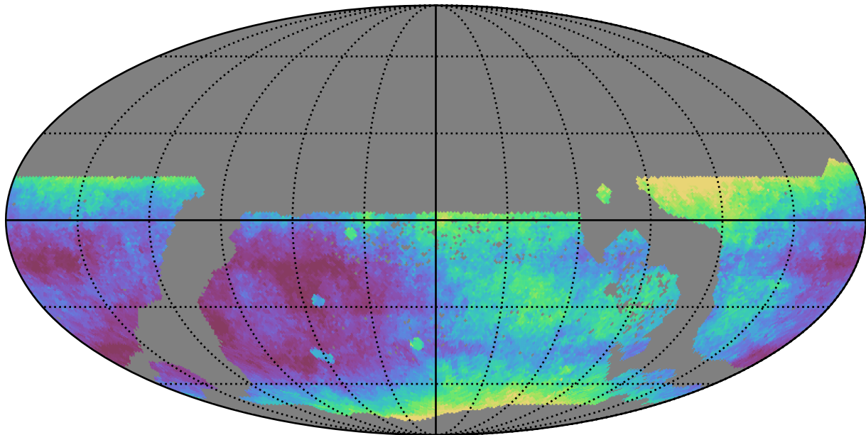
too_elab_r8_d2_gz_v3.4_10yrs WFD r band: Median seeingEff
