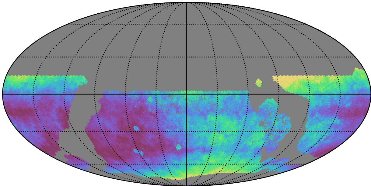
too_elab_r8_d2_gz_v3.4_10yrs WFD i band: Median seeingEff
