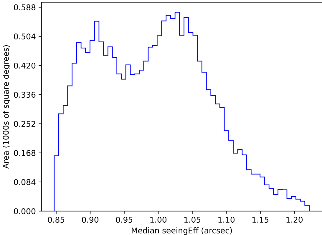
too_elab_r8_d2_gz_v3.4_10yrs WFD i band: Median seeingEff
