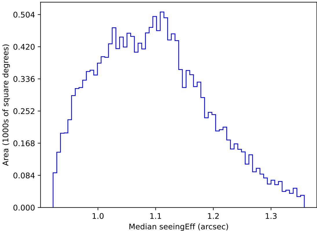
too_elab_r8_d2_gz_v3.4_10yrs WFD g band: Median seeingEff
