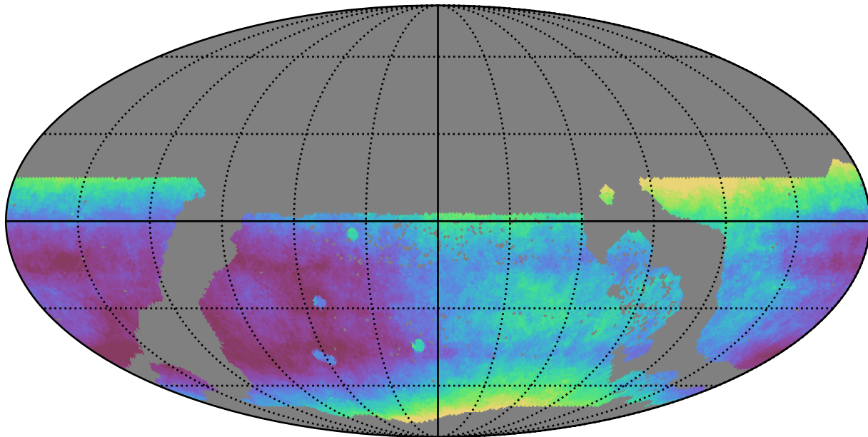
too_elab_r8_d2_gz_v3.4_10yrs WFD all bands: Median seeingEff
