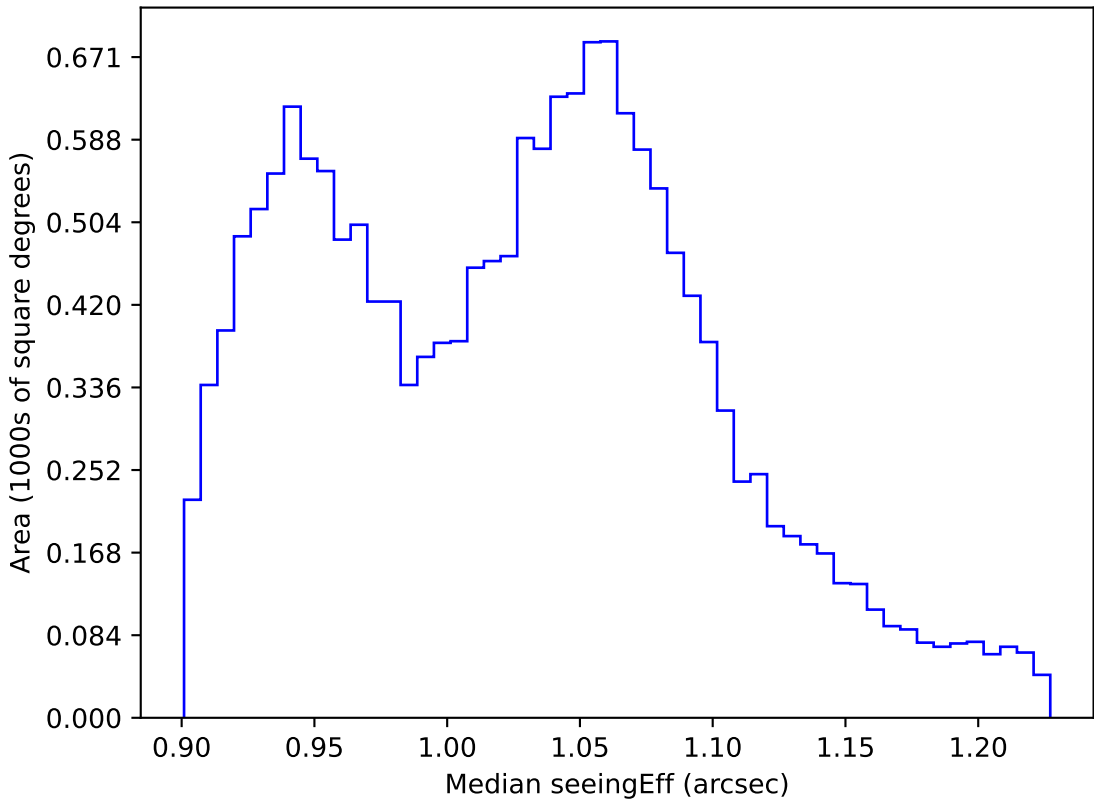
too_elab_r8_d2_gz_v3.4_10yrs WFD all bands: Median seeingEff
