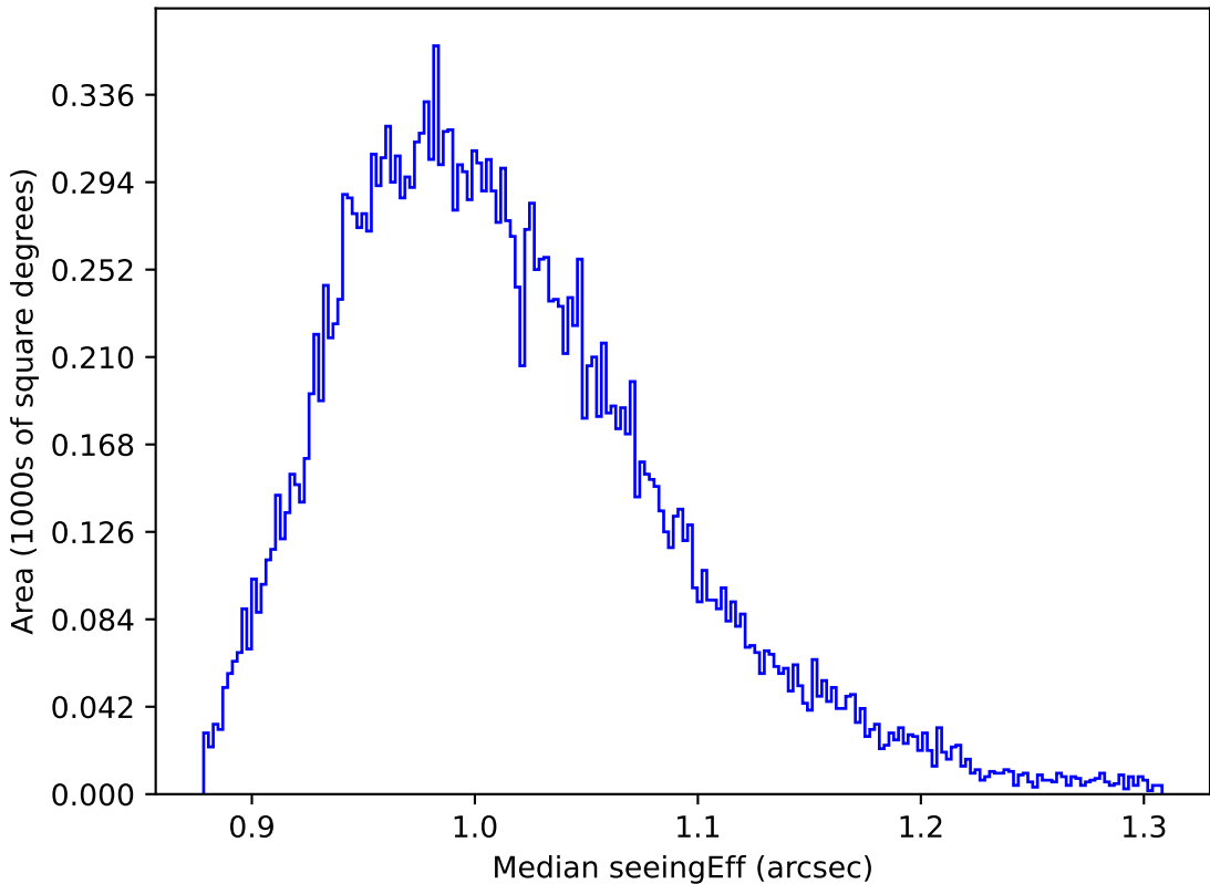
too_elab_r8_d2_gz_v3.4_10yrs All sky y band: Median seeingEff
