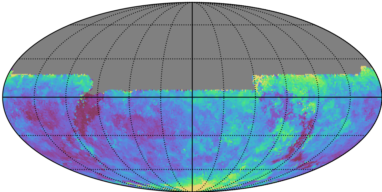
too_elab_r8_d2_gz_v3.4_10yrs All sky u band: Median seeingEff
