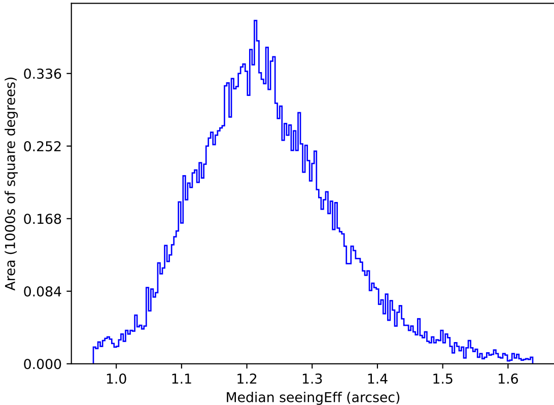
too_elab_r8_d2_gz_v3.4_10yrs All sky u band: Median seeingEff
