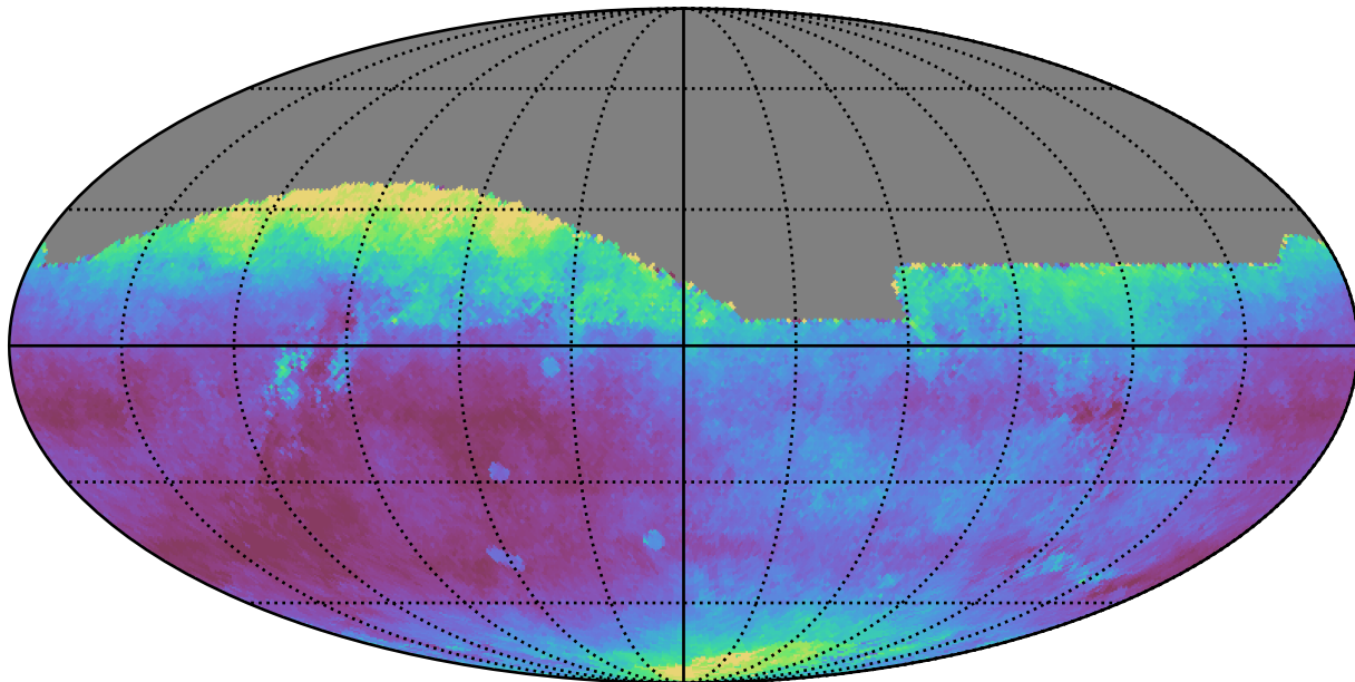
too_elab_r8_d2_gz_v3.4_10yrs All sky r band: Median seeingEff
