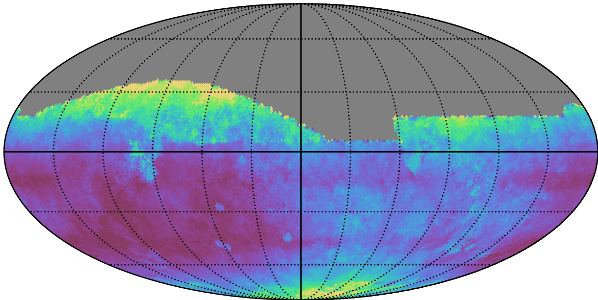
too_elab_r8_d2_gz_v3.4_10yrs All sky i band: Median seeingEff
