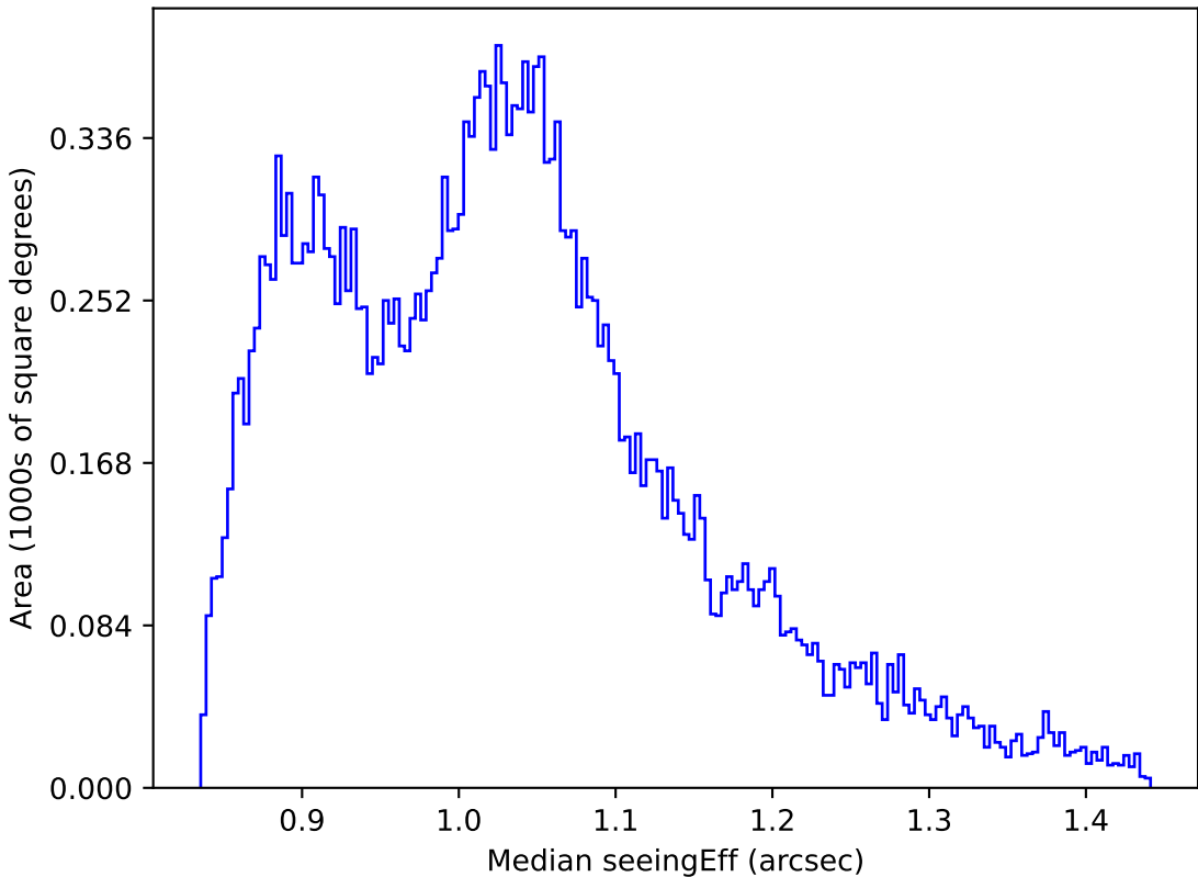
too_elab_r8_d2_gz_v3.4_10yrs All sky i band: Median seeingEff
