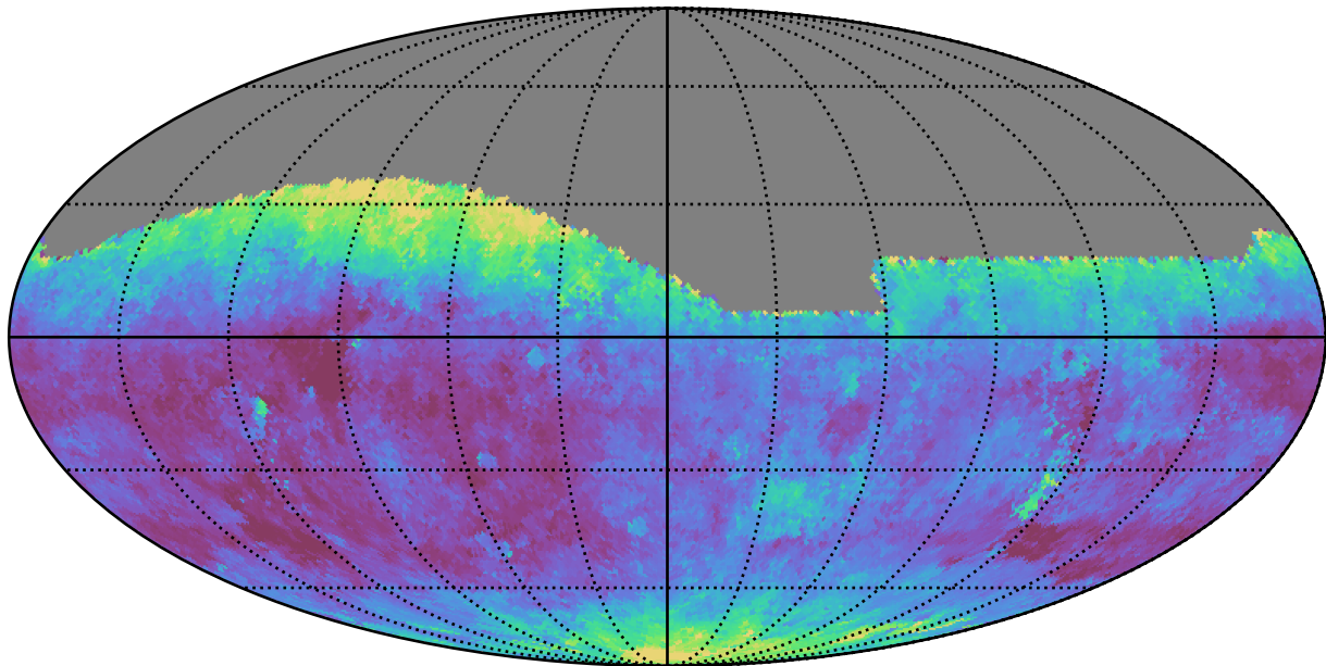
too_elab_r8_d2_gz_v3.4_10yrs All sky g band: Median seeingEff
