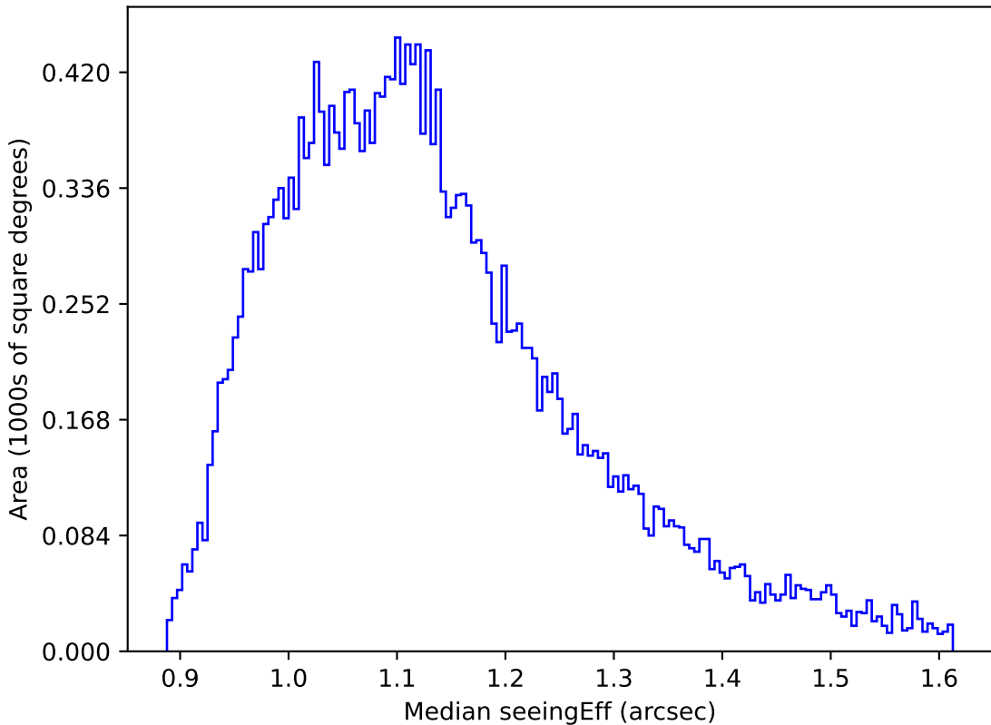
too_elab_r8_d2_gz_v3.4_10yrs All sky g band: Median seeingEff
