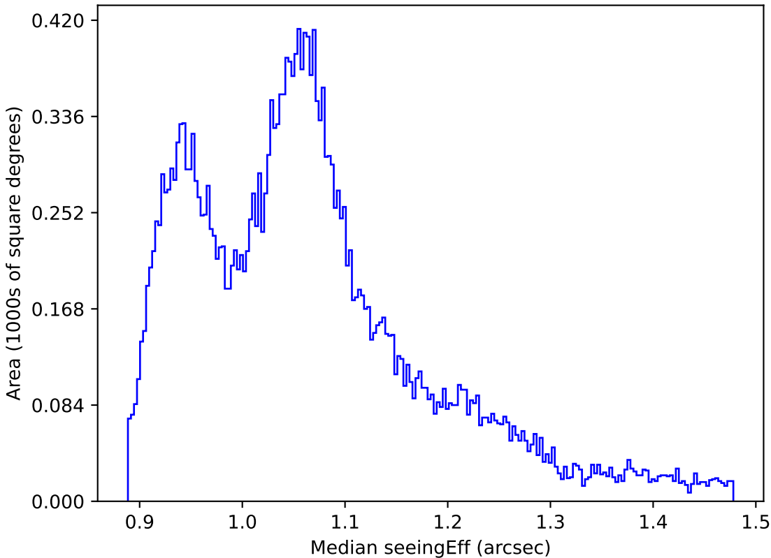
too_elab_r8_d2_gz_v3.4_10yrs All sky all bands: Median seeingEff
