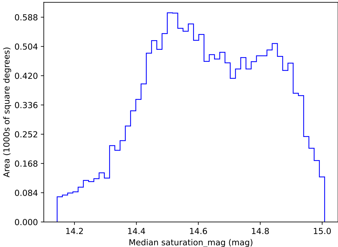
too_elab_r8_d2_gz_v3.4_10yrs WFD r band: Median saturation_mag
