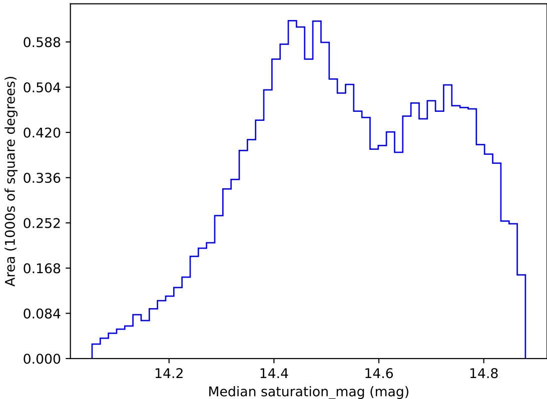
too_elab_r8_d2_gz_v3.4_10yrs WFD i band: Median saturation_mag
