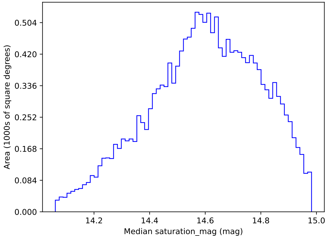
too_elab_r8_d2_gz_v3.4_10yrs WFD g band: Median saturation_mag
