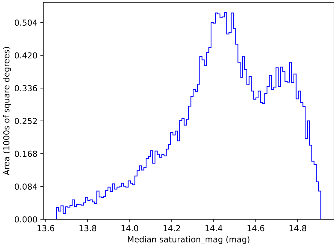
too_elab_r8_d2_gz_v3.4_10yrs All sky i band: Median saturation_mag
