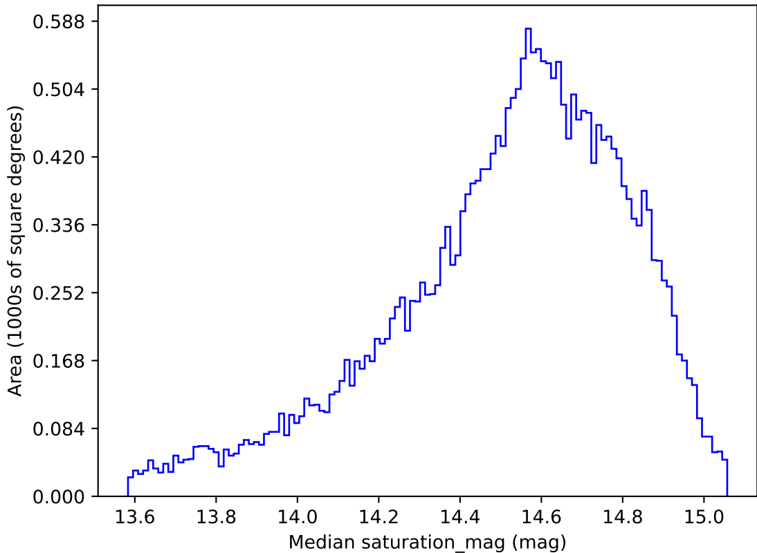
too_elab_r8_d2_gz_v3.4_10yrs All sky g band: Median saturation_mag
