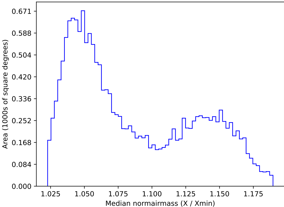
too_elab_r8_d2_gz_v3.4_10yrs WFD z band: Median normairmass
