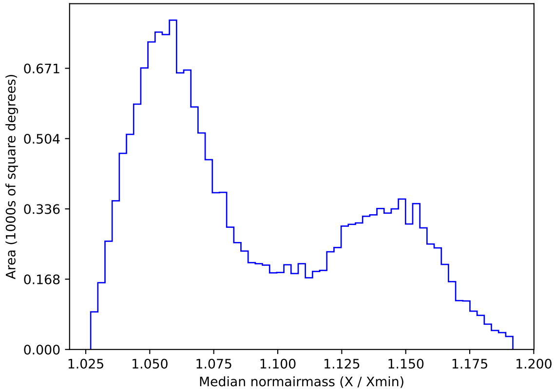
too_elab_r8_d2_gz_v3.4_10yrs WFD y band: Median normairmass
