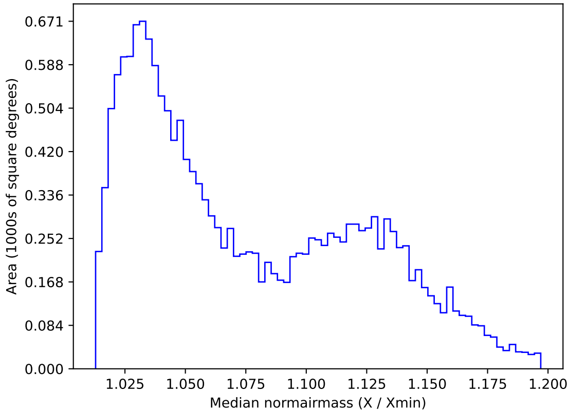
too_elab_r8_d2_gz_v3.4_10yrs WFD u band: Median normairmass
